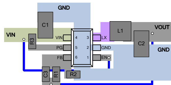
Figure 17. Recommended Layout Diagram
