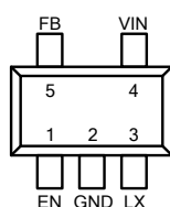
Figure 1. Pin Assignment of FP6396
