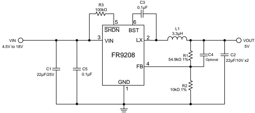
Figure 2. FR9208 Application Circuit
