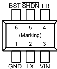
Figure 1. Pin Assignments of FR9208
