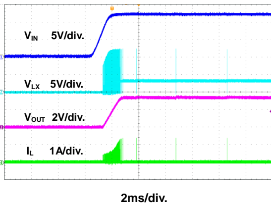
Figure 12. Startup Through Power Supply Waveform
