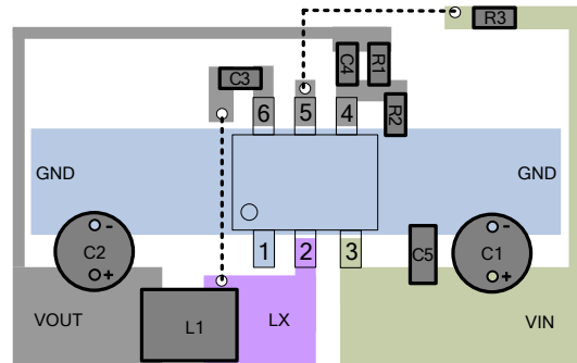
Figure 21. Recommended PCB Layout Diagram
