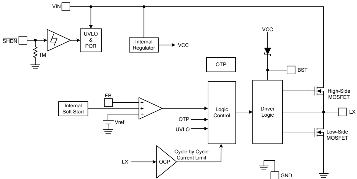
Figure 3. Block Diagram of FR9208
