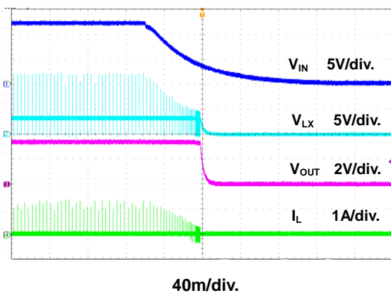
Figure 14. Shutdown Through Power Supply Waveform
