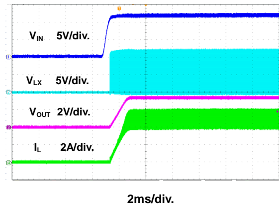
Figure 13. Startup Through Power Supply Waveform
